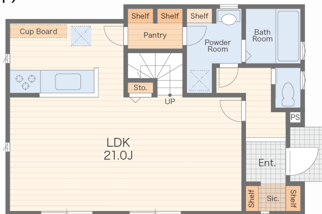
1F
